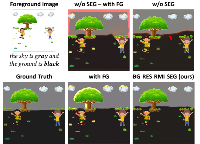
Fig. 15. Illustration of the advantages of the segmentation branch of the proposed architecture and the w/o-FG training strategy for background colorization.
